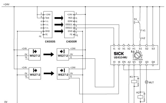
Connection diagram
