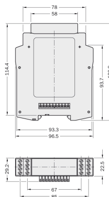
Dimensional drawing
