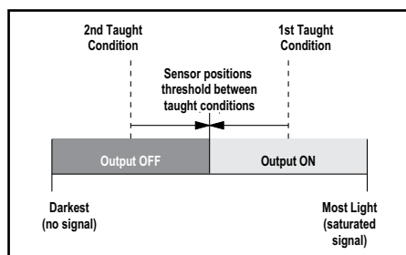
Figure 3. Static TEACH (Light Operate shown)
