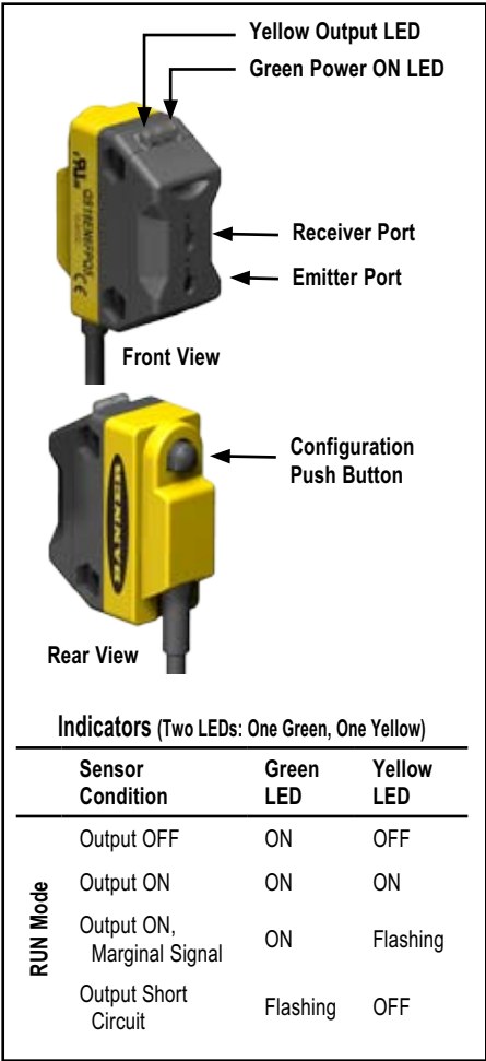
Figure 1. Features — fiber optic model shown
