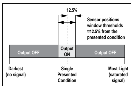
Figure 7. Window SET (Light Operate shown)
