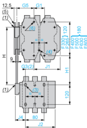
Assembly B (7) - Mechanical interlock reference
