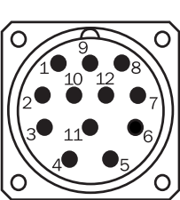
View of M23 device connector on cable/housing
