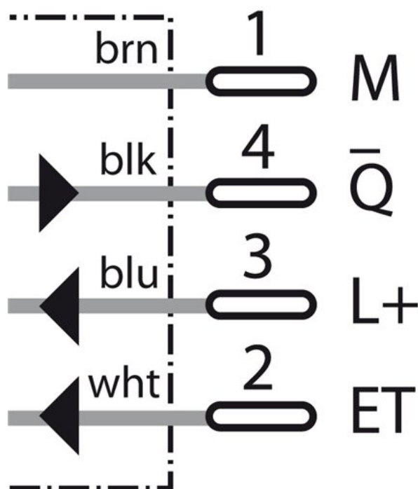
Connection diagram
