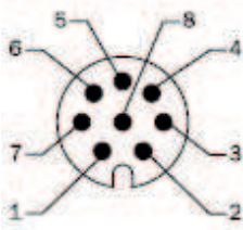
View of M12 device connector on encoder
