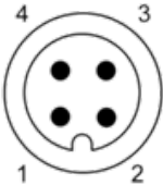
4-Wire DC, PNP/NPN, NO or NC output
