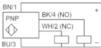
PNP 4-wire
